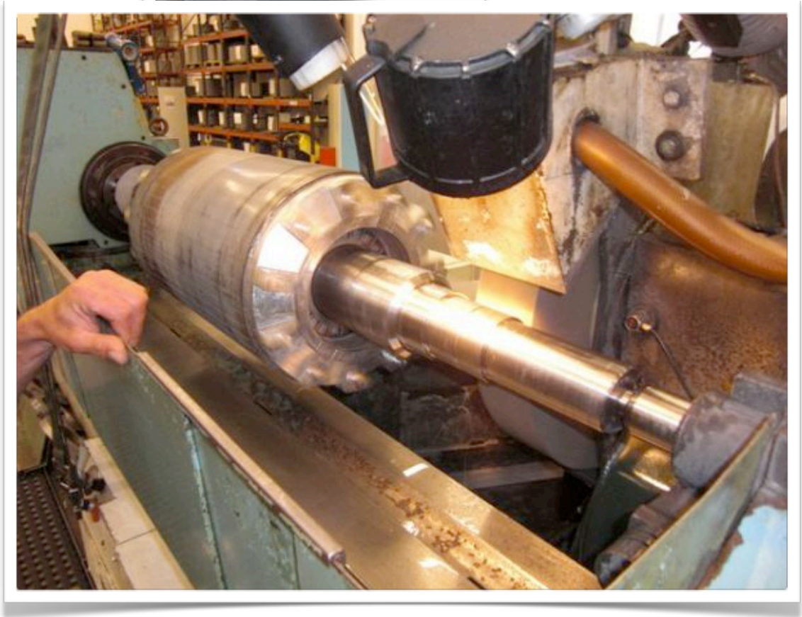
TACHELLA UMP 2628 CYLINDRICAL GRINDER
